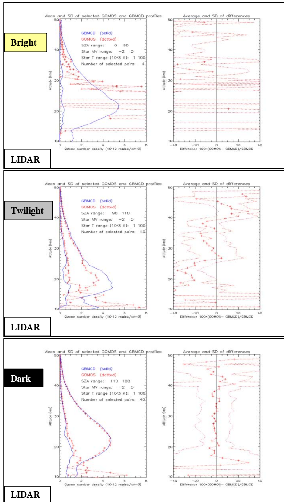
Fig. 2. Analysis of lidar compared to GOMOS ozone profiles with respect to the SZA during GOMOS observation. Top, middle, and bottom panel show the results for bright, twilight, and dark conditions respectively. Left plots show the mean ozone profiles and their standard deviation. Right plots show average differences between GOMOS and GBMCD profiles and std. deviation in percentage relative to the latter.
