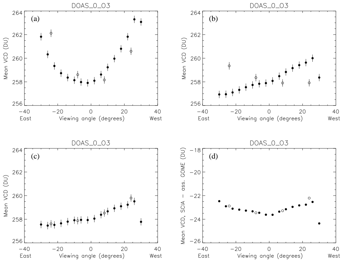
Figure 6: Mean ozone vertical column density as a function of viewing angle for all pixels with 1/4 second integration time from 25 October until 6 November (SV 3.53): (a) from level-2 product, (b) with viewing angle corrected for top-of-atmosphere, (c) with correction for viewing angle shift, (d) with assimilated GOME column subtracted. Filled dots are forward-scan pixels; open dots are backscans. The error bars reflect \pm\sigma/n^{1/2} , where n is the number of pixels on which the mean vertical column is based and \sigma the standard deviation.
