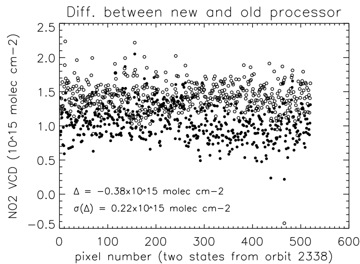
Figure 8: As Fig. 5 but for NO 2 .
